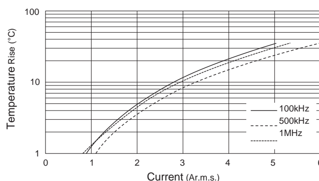
Ripple Current
