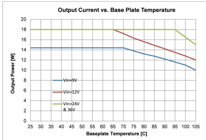
Fig. 15: ICH0518V1PC Derating Curve (I out )
