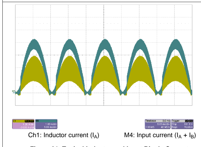
Figure 31. Typical Inductor and Input Ripple Currents
