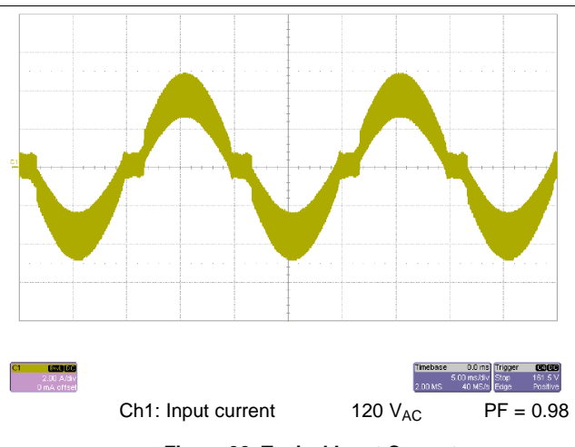
Figure 32. Typical Input Current
