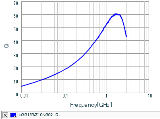
Q-Frequency Characteristics
