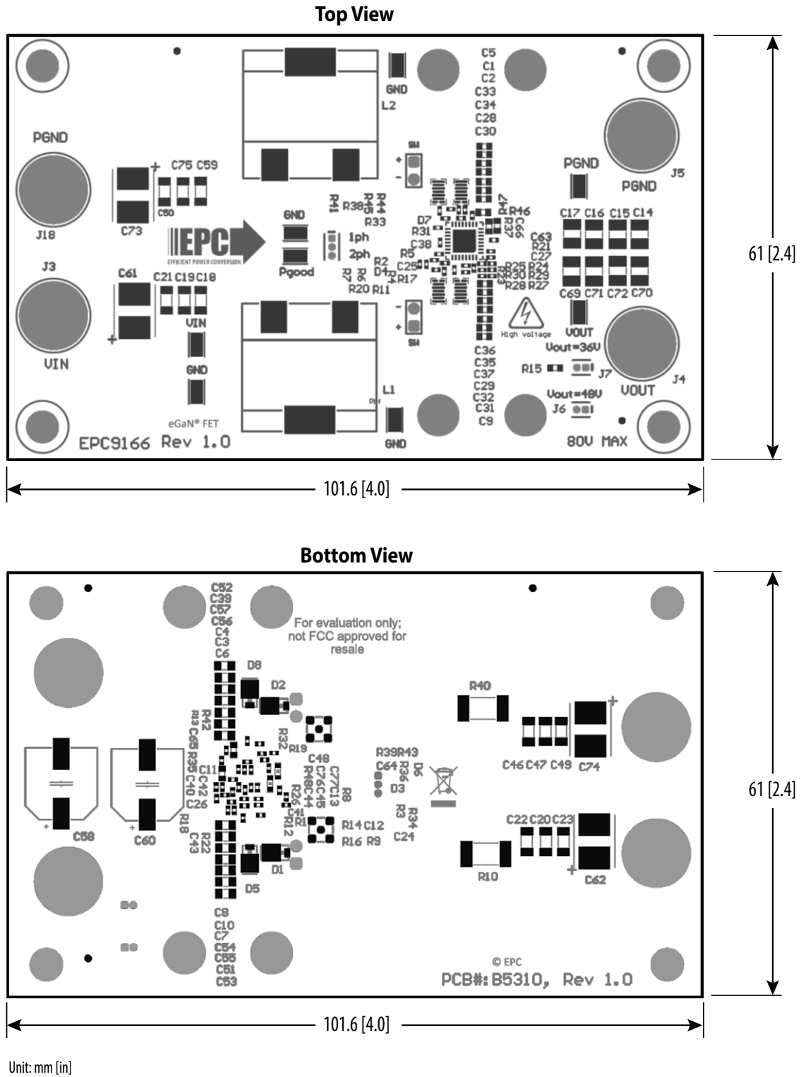
Figure 12: Mechanical dimensions
