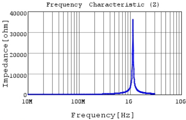
LQG15WHR13G02 |Z|
