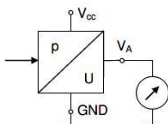
3-wire connection (standard)
