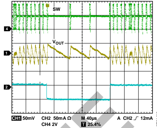
Figure 18. Load Transient, V_{OUT} = 1.8V, 5mA to 50mA
