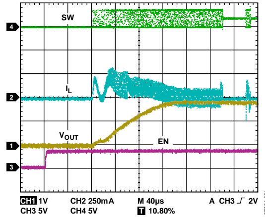
Figure 20. Startup, V_{OUT} = 1.8V, 5mA
