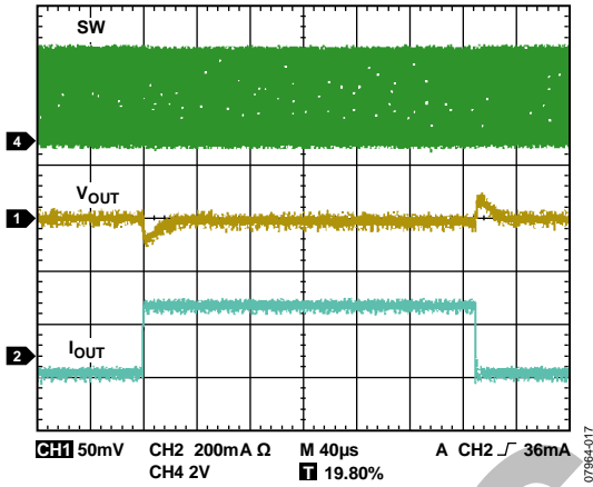
Figure 16. Load Transient, V_{OUT} = 1.8V, 300mA to 600mA
