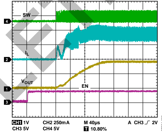
Figure 19. Startup, V_{OUT} = 1.8V, 400mA
