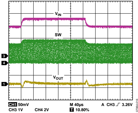
Figure 15. Line Transient, V_{OUT} = 1.0V
