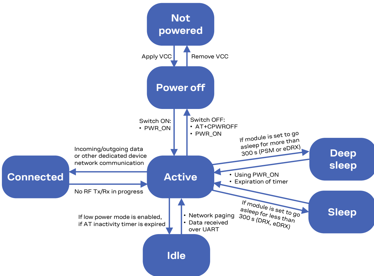
Figure 4: SARA-N3 series modules' operating modes transitions
