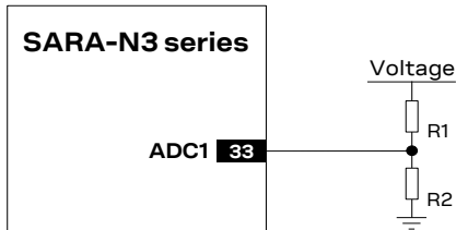
Figure 46: ADC application circuit example
