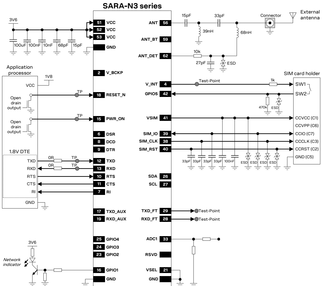
Figure 50: Sample schematic diagram to integrate a SARA-N3 “00” product version using most of the interfaces
