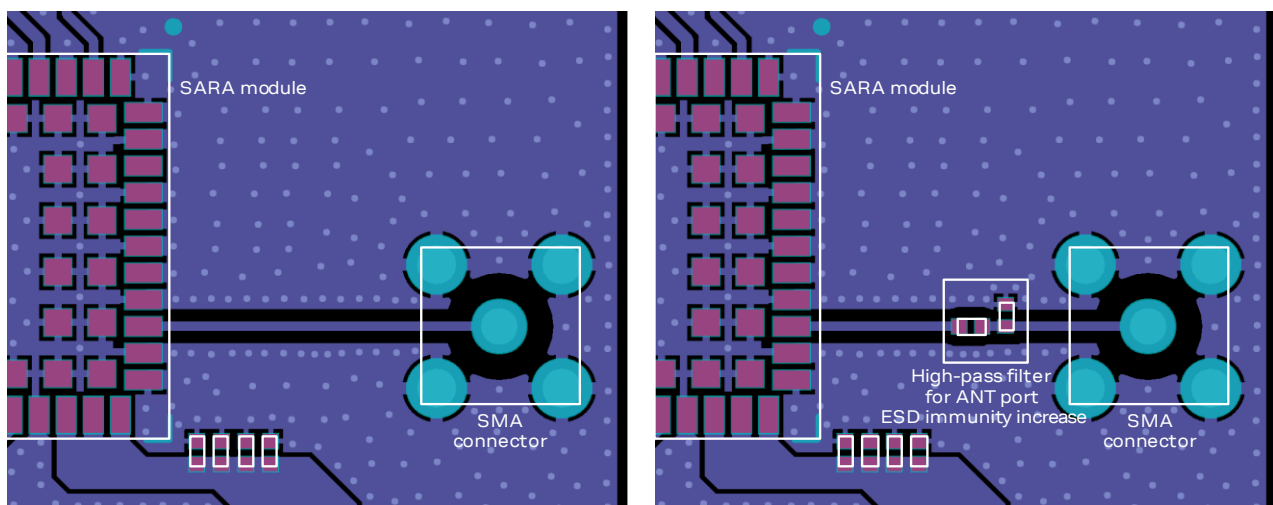
Figure 27: Suggested circuit and layout for antenna RF circuit on application board, if antenna detection is not required
