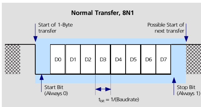
Figure 12: Description of UART default frame format (8N1) with fixed baud rate
