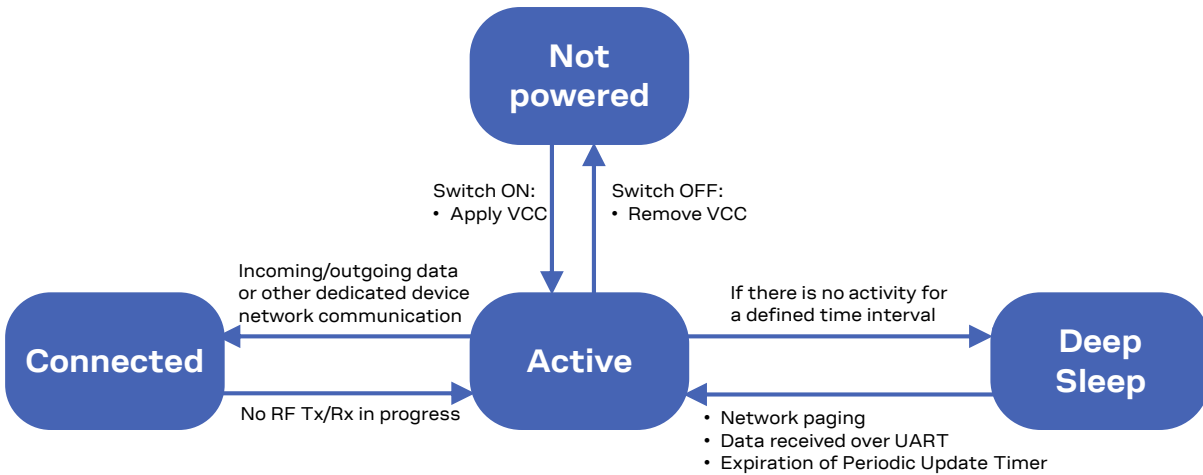
Figure 3: SARA-N2 series modules' operating modes transitions
