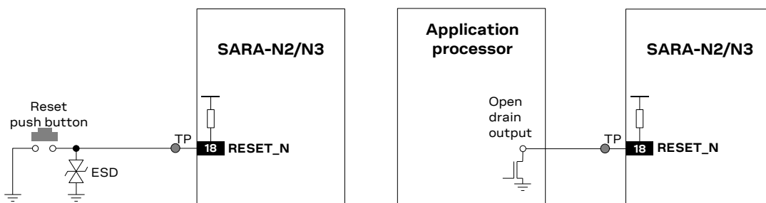
Figure 21: RESET_N application circuits using a push button and an open drain output of an application processor
