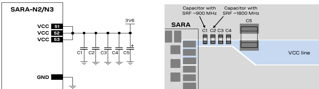
Figure 18: Suggested schematic and layout design for the VCC line, highly recommended when using an integrated antenna
