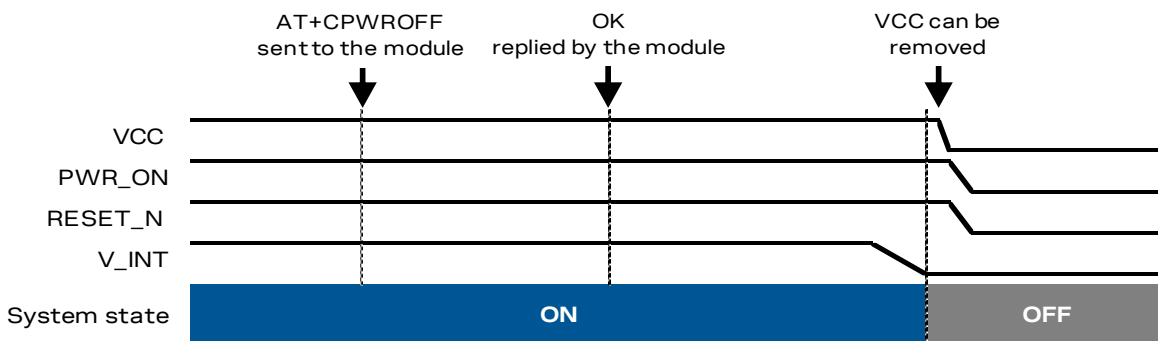
Figure 10: SARA-N3 series modules switch-off sequence by means of AT+CPWROFF command
