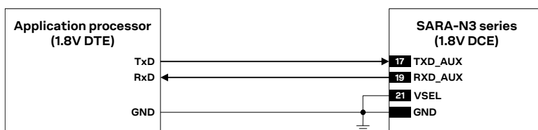
Figure 42: SARA-N3 series' UART AUX application circuit with TXD_AUX / RXD_AUX lines connection (1.8 V DTE / 1.8 V DCE)
