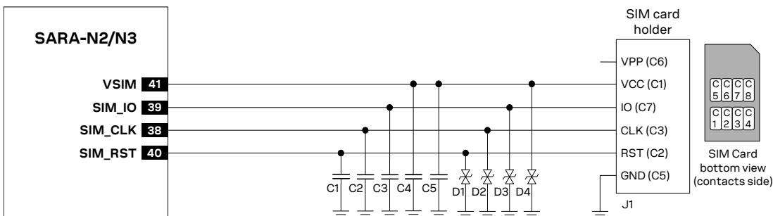
Figure 30: Application circuit for the connection to a single removable SIM card
