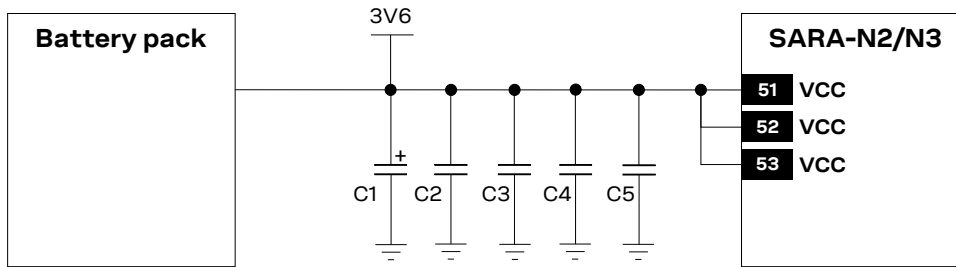
Figure 14: Suggested schematic design for the VCC voltage supply application circuit using a LiSOCl 2 primary battery
