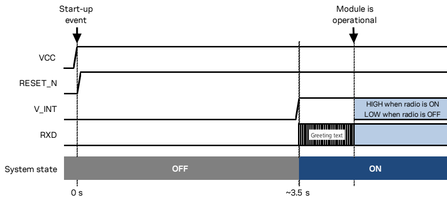
Figure 8: SARA-N2 series power-on sequence from not-powered mode
