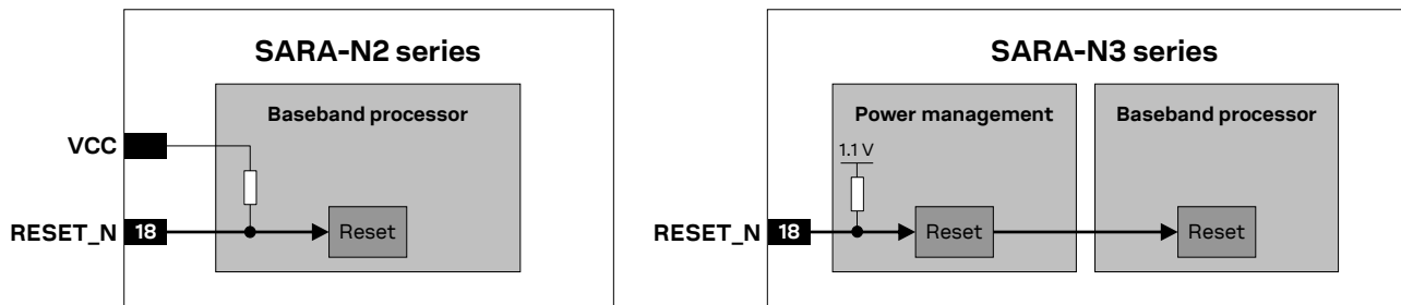
Figure 11: SARA-N2 / N3 series RESET_N input equivalent circuit description
