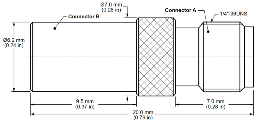
Figure 1. Product Dimensions for the ADP-SMAF-SMBM-G Adapter
