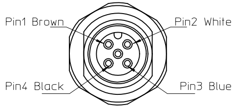
FRON SIDE VIEW FEMALE 4 POLE
