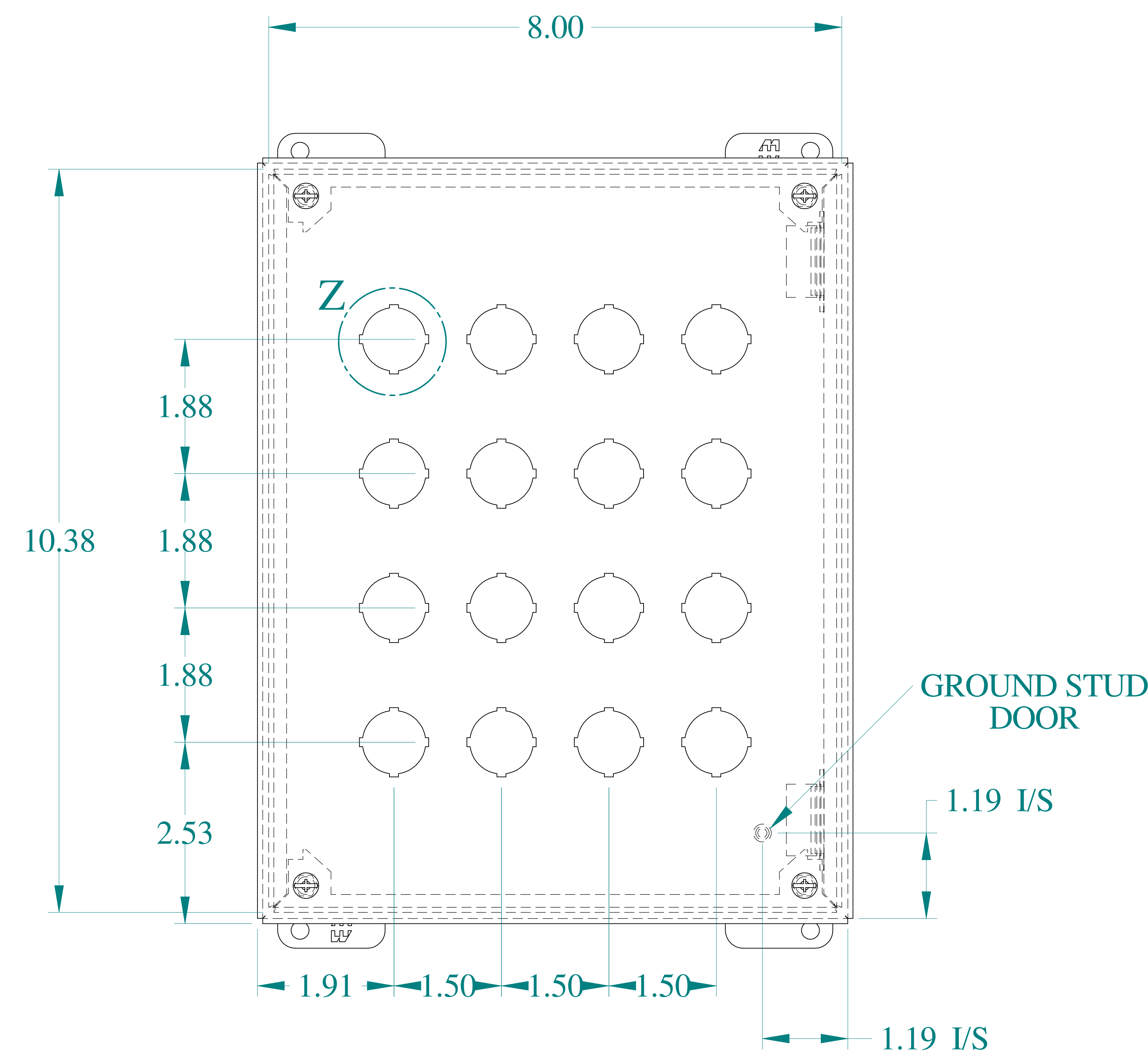
FRONT VIEW
