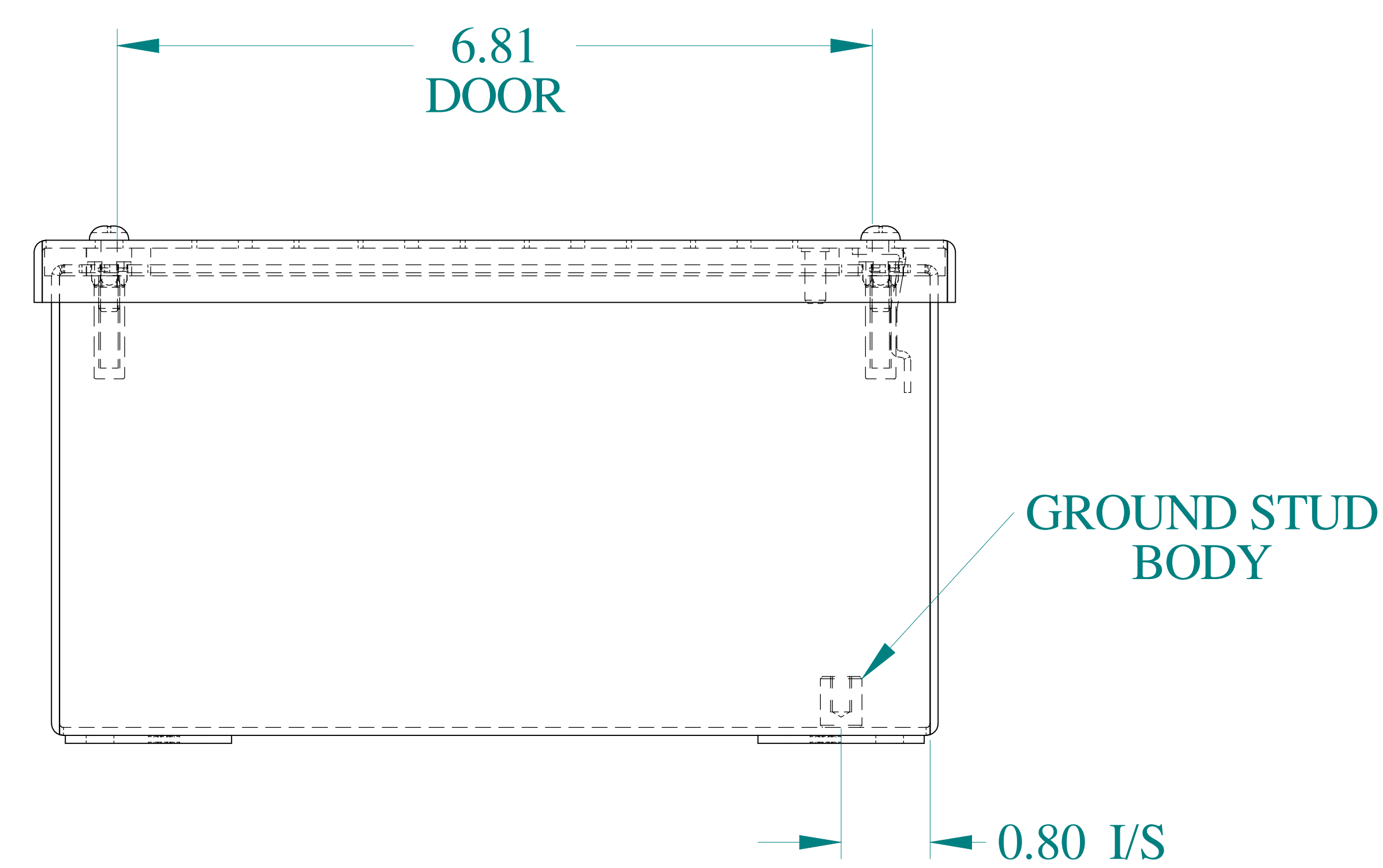
BOTTOM VIEW
