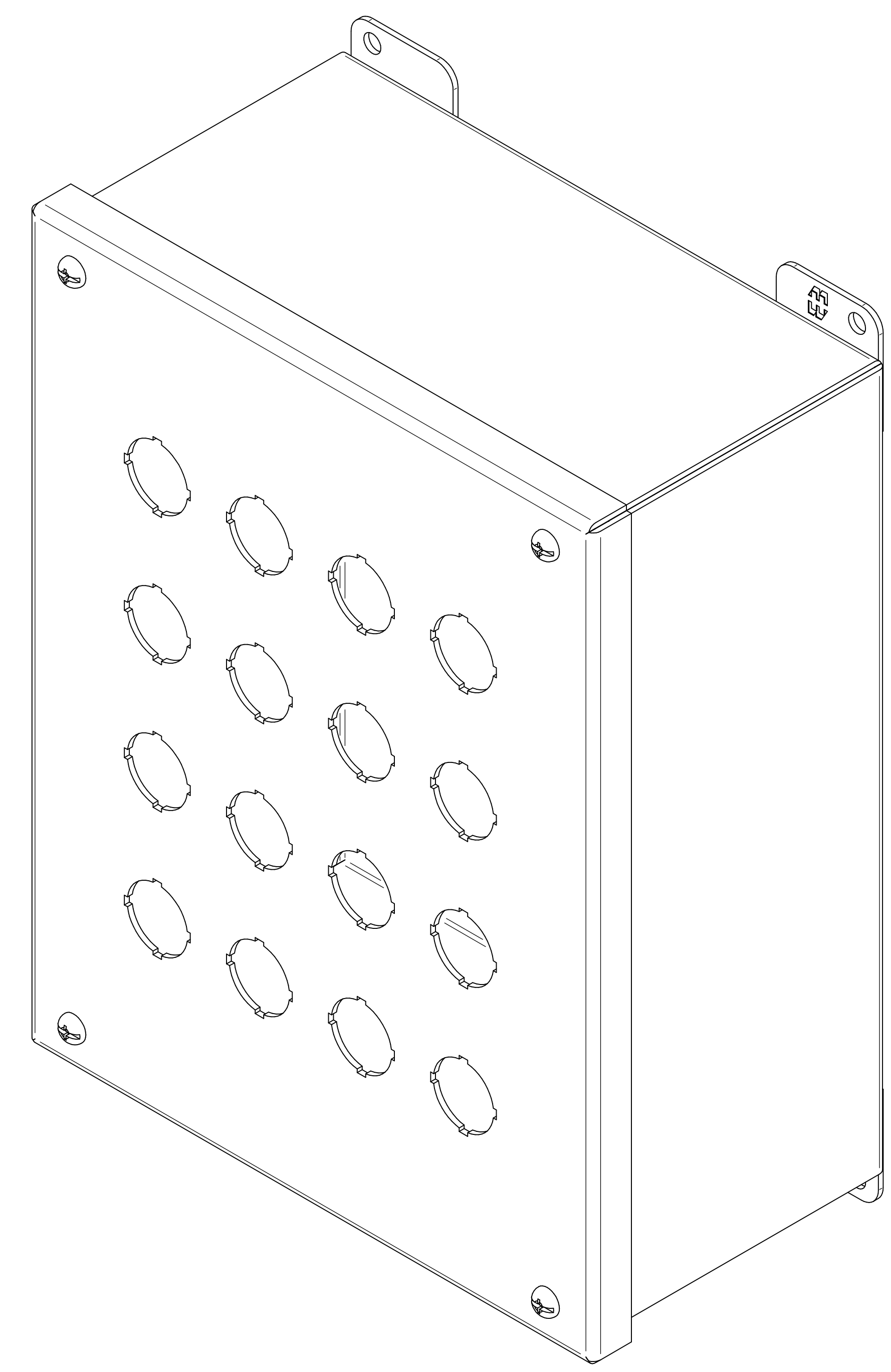
ISOMETRIC VIEWS
