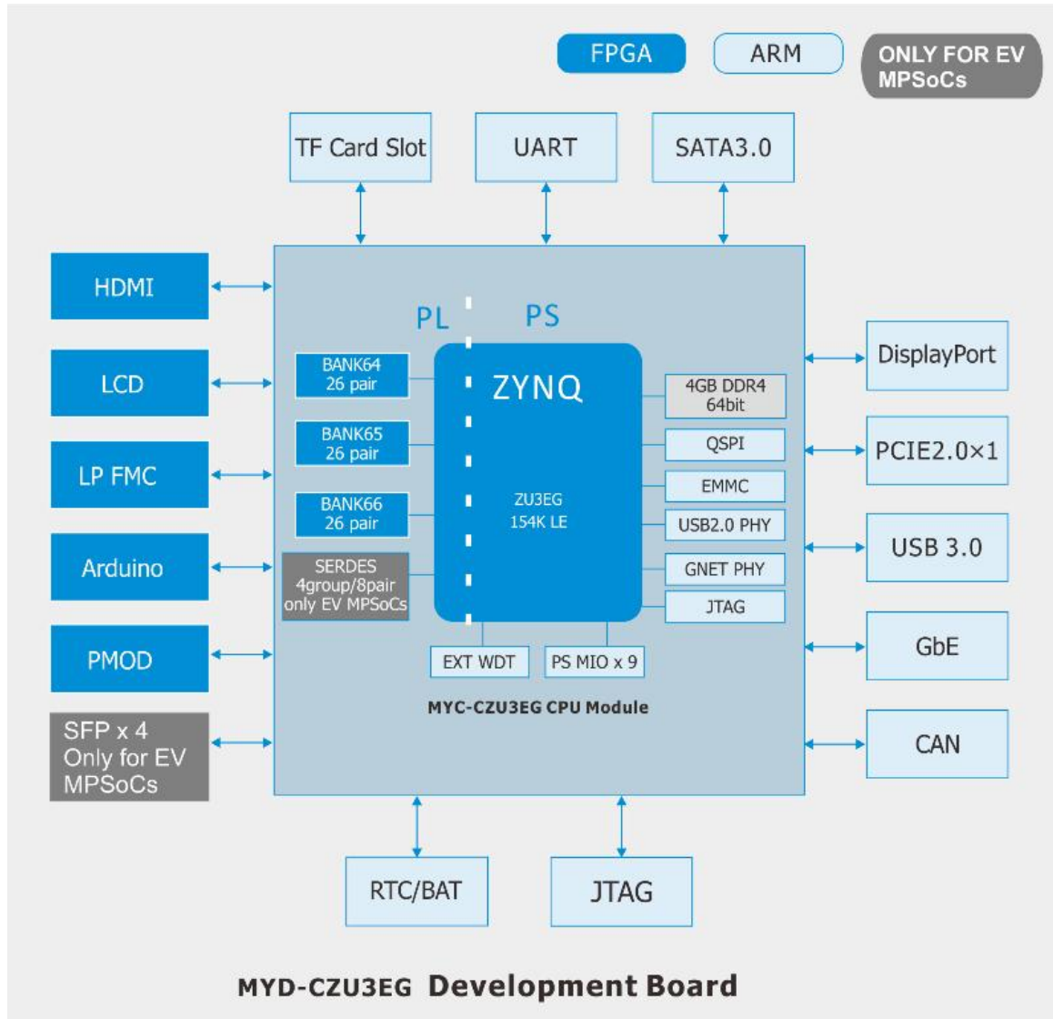
Figure 1-9 Function Block Diagram of MYD-CZU3EG/4EV/5EV-V2
