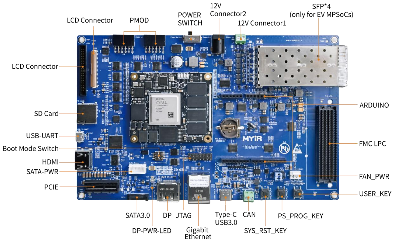
Figure 1-2 MYD-CZU3EG/4EV/5EV-V2 Development Board
