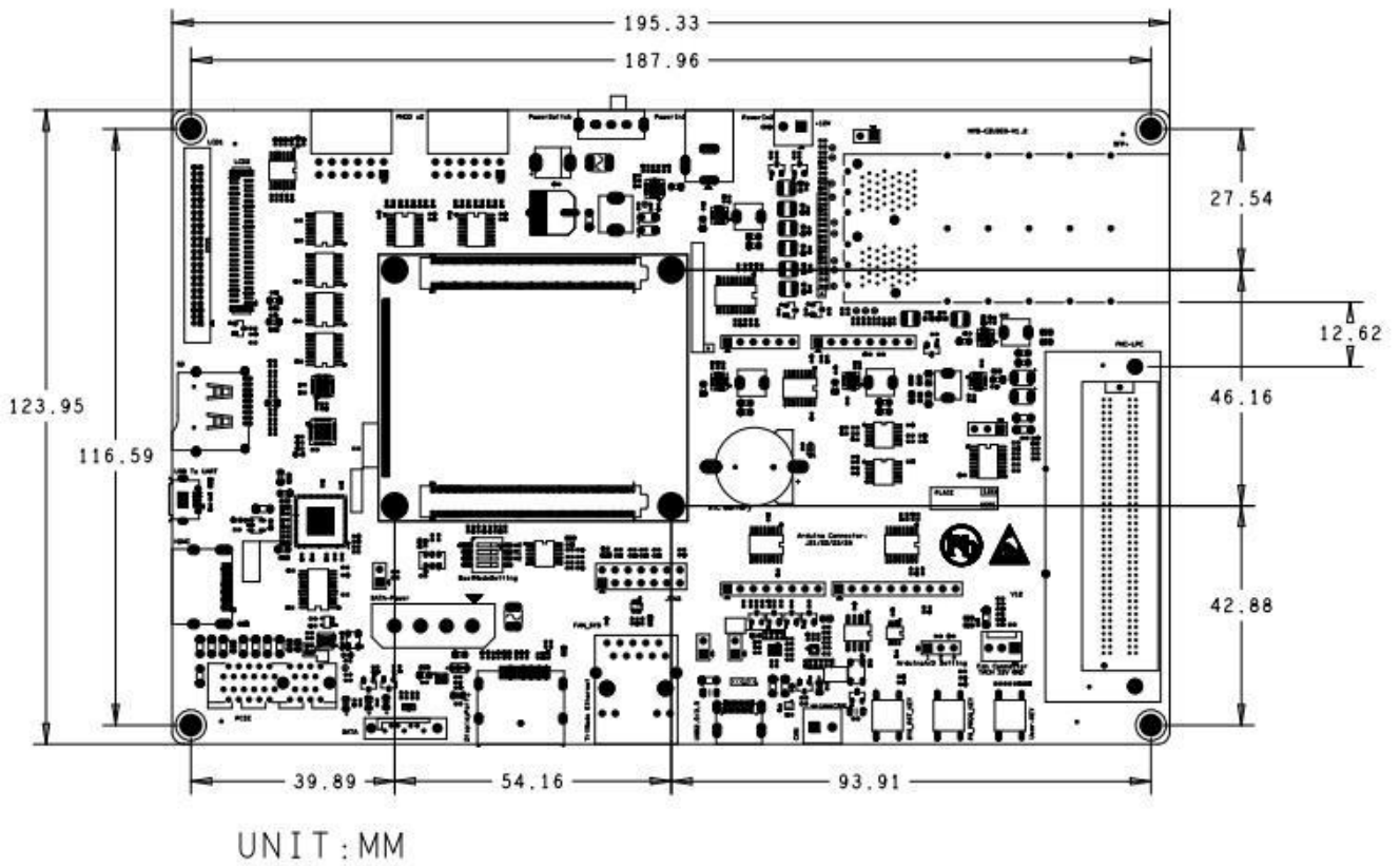
Figure 1-11 Dimension Chart of MYD-CZU3EG/4EV/5EV-V2
