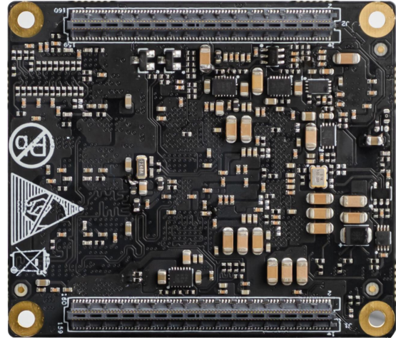
Figure 1-7 MYC-CZU3EG/4EV/5EV-V2 Bottom-view
