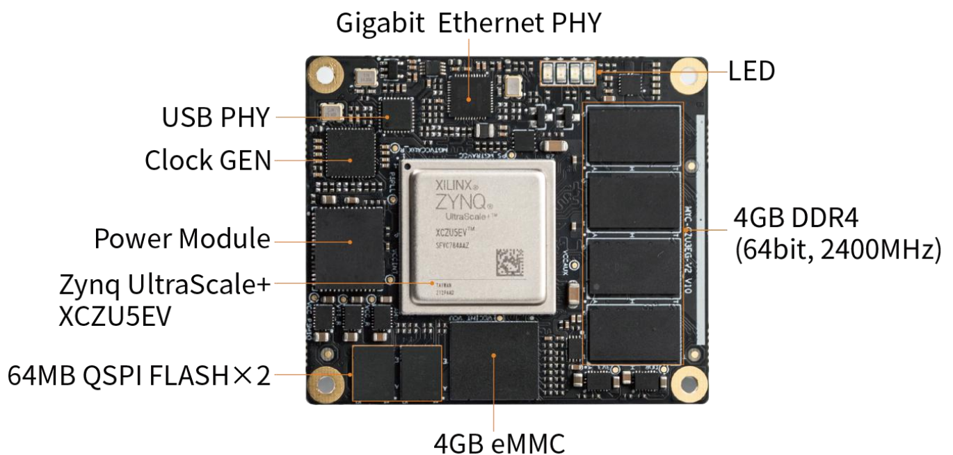
Figure 1-3 MYC-CZU3EG/4EV/5EV-V2 CPU Module
