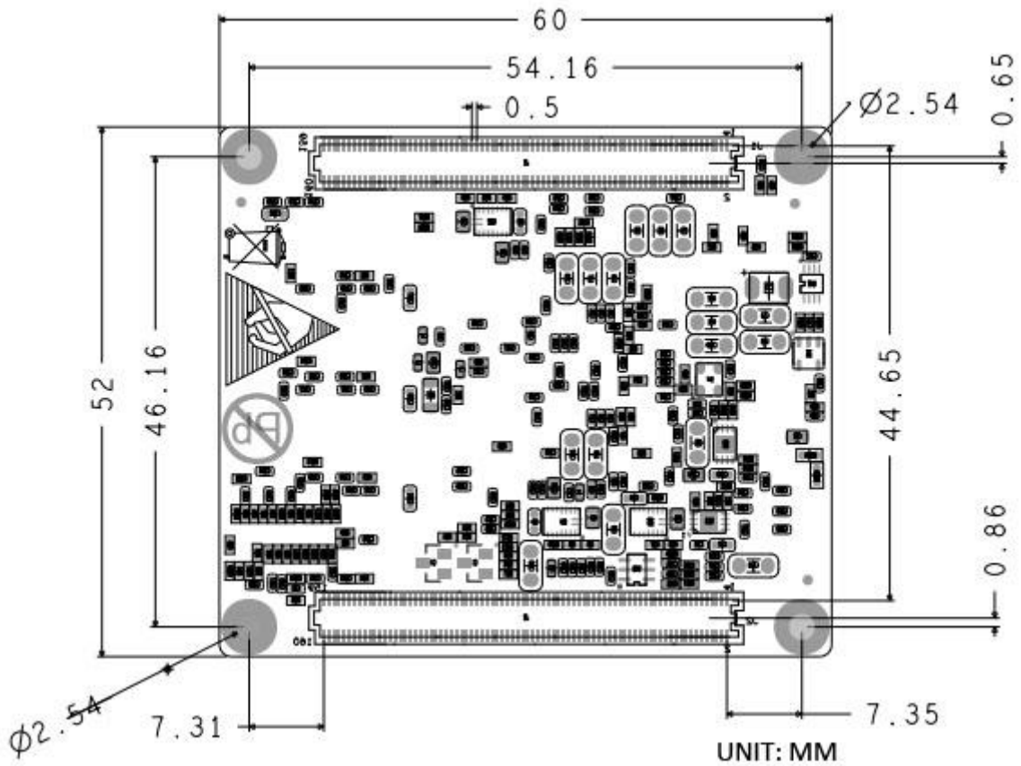
Figure 1-10 Dimension Chart of MYC-CZU3EG/4EV/5EV-V2 (Top-view)
