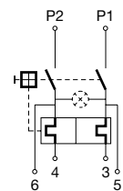
2 pole thermal overload protection, Shunt terminal
