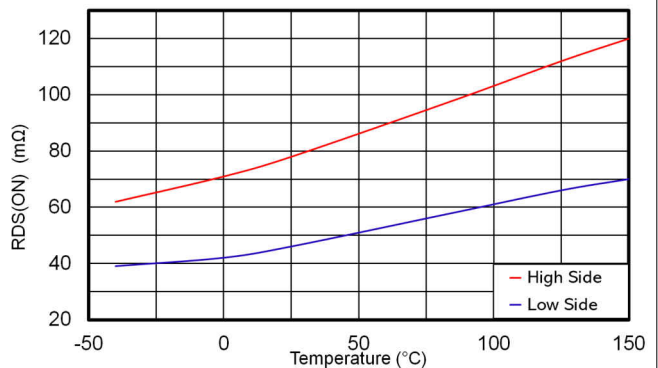
Figure 7-12. High Side and Low Side Switches R DS_ON
