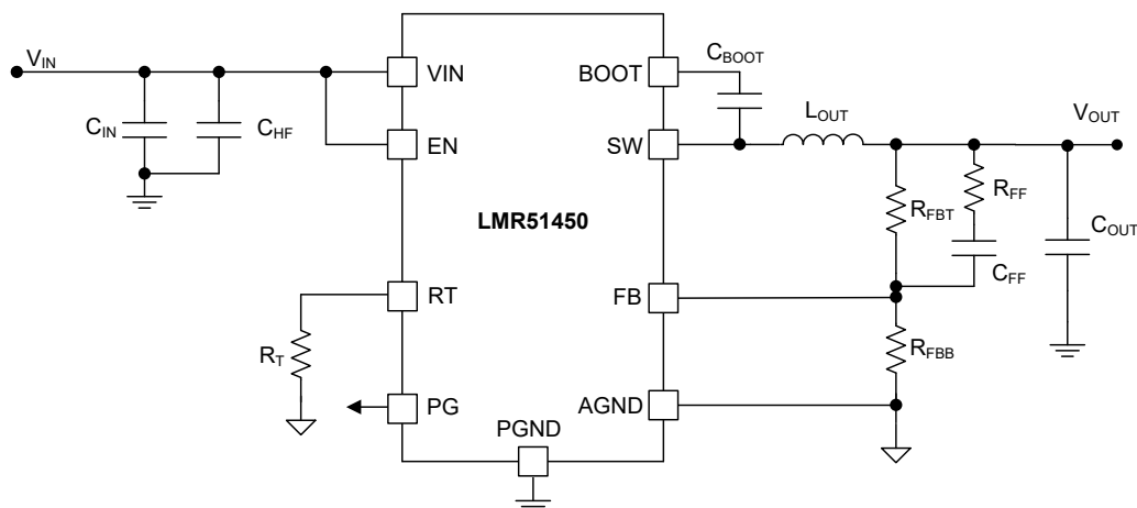
Figure 9-1. Application Circuit
