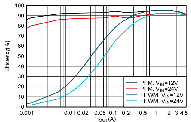
Efficiency vs Output Current V OUT = 5 V, 500 kHz
