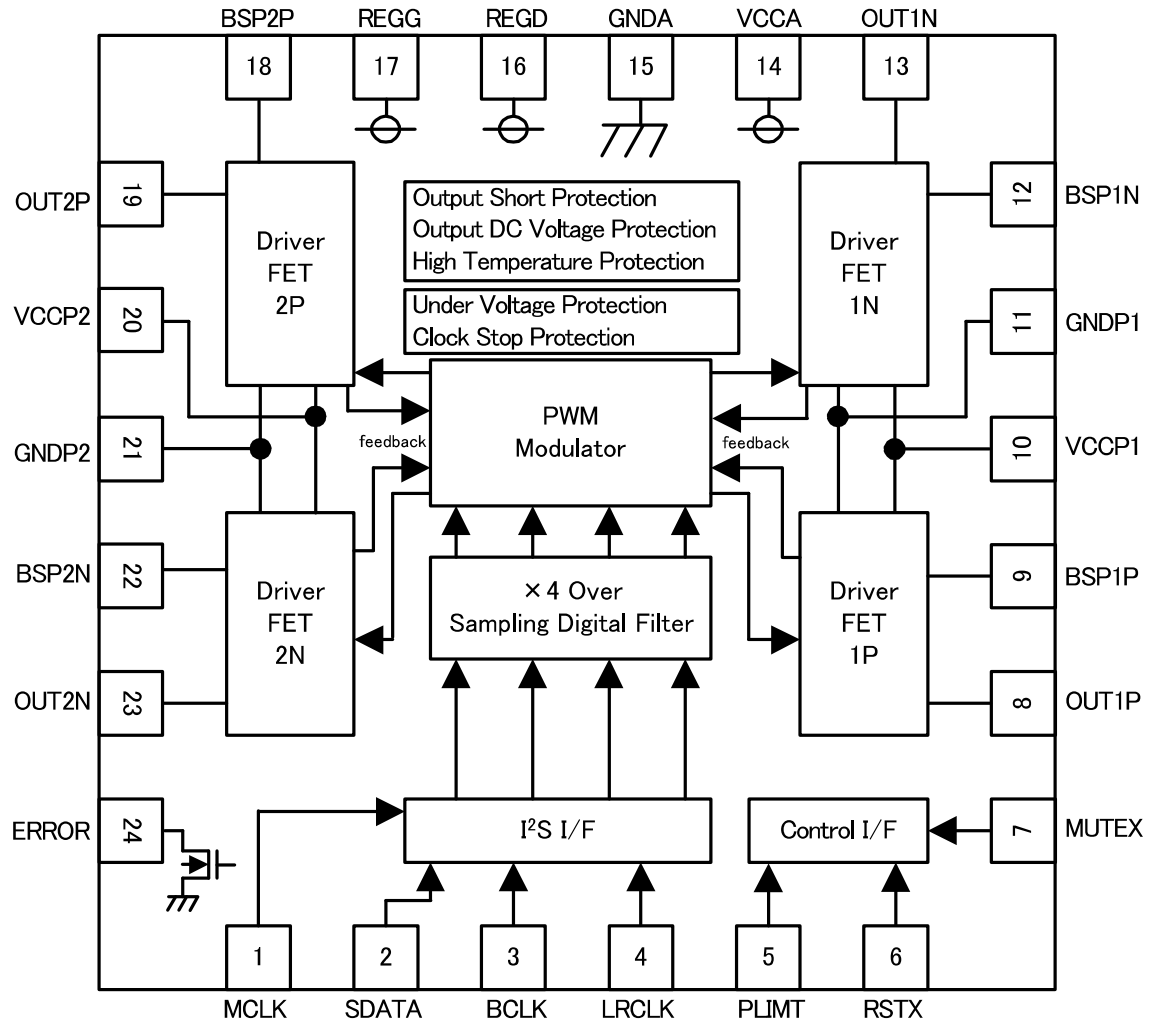
Figure 3. Block Diagram
