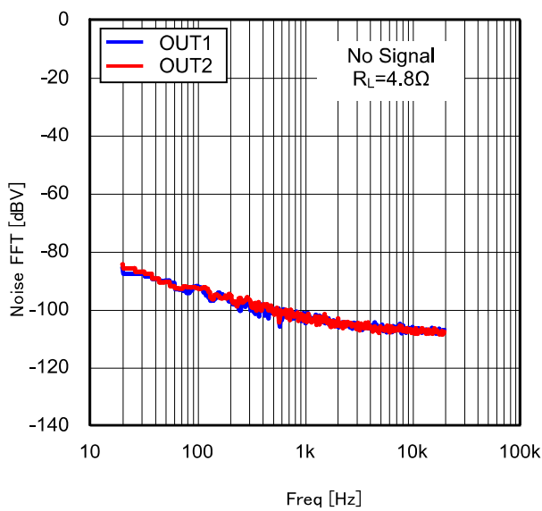
Figure 39. FFT of output noise voltage ( 4.8\Omega )
