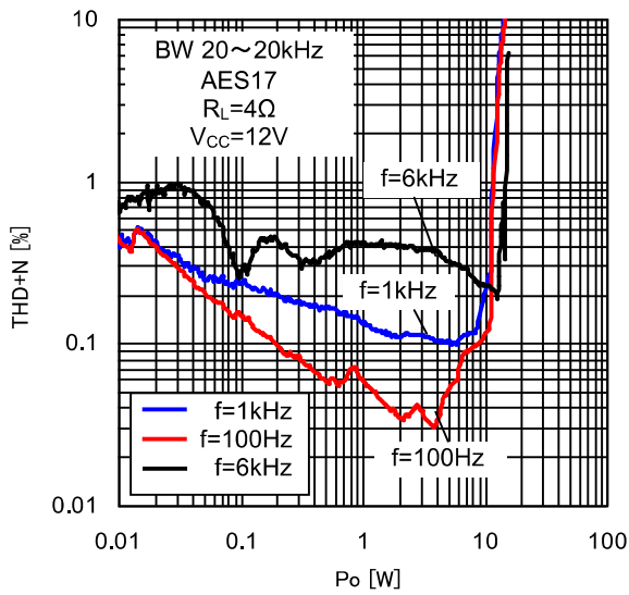
Figure 35. THD+N vs P_O (4 \Omega )
