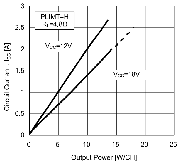
Figure 20. Circuit Current vs Output Power (4.8Ω)
