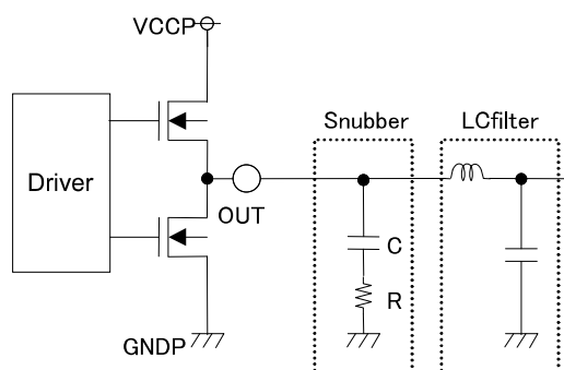
Figure74. Snubber Schematic
