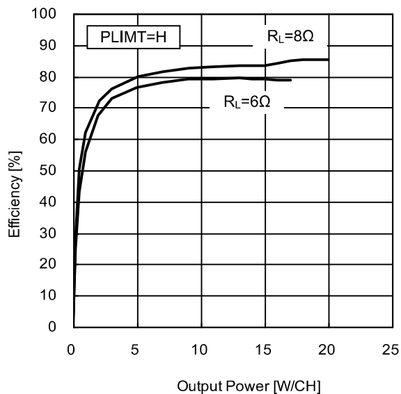
Figure 7. Efficiency vs Output Power (8Ω, 6Ω)
