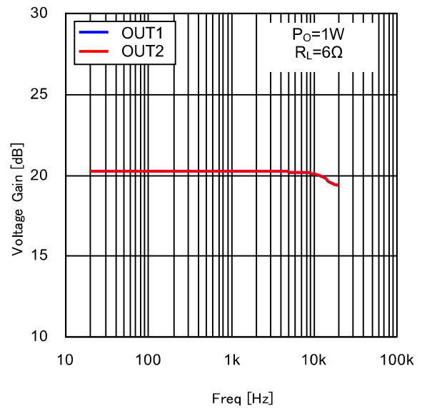
Figure 28. Voltage Gain vs Freq ( 6\Omega )
