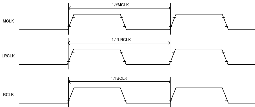
Figure 57. Clock Timing
