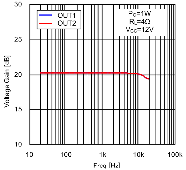
Figure 34. Voltage Gain vs Freq (4 \Omega )
