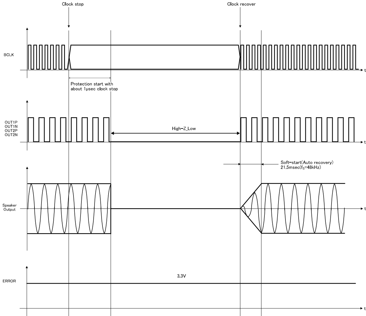
Figure 67. Clock Stop Protection (BCLK) Sequence
