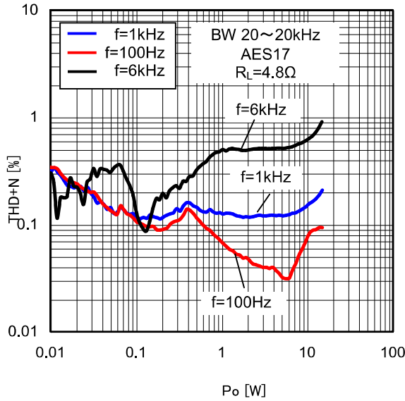
Figure 41. THD+N vs P_o (4.8 \Omega )
