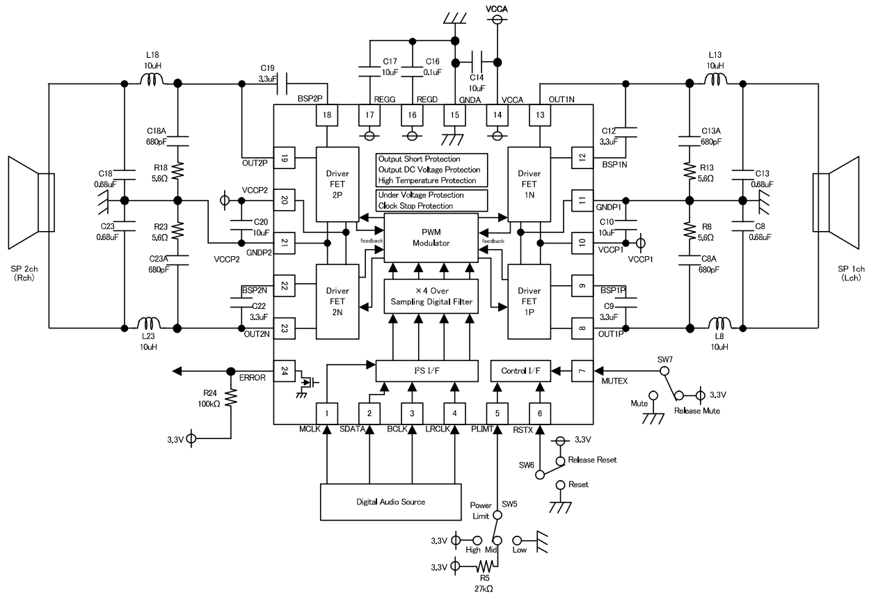
Figure 69. Application Circuit
