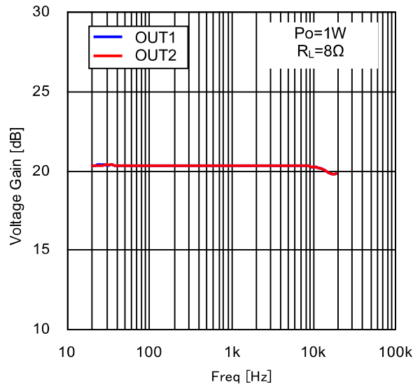
Figure 22. Voltage Gain vs Freq (8 \Omega )
