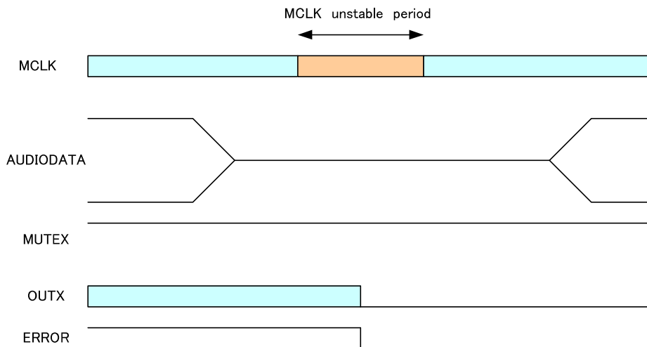
Figure 50. Action at MCLK Unstable 1
