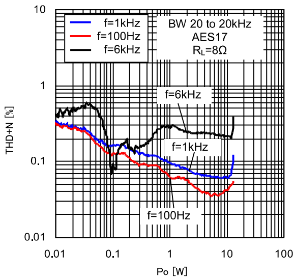
Figure 23. THD+N vs P_o (8 \Omega )
