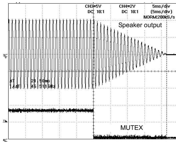
Figure 12. Waveform of Soft Mute
