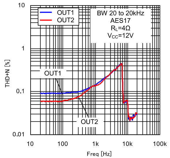
Figure 36. THD+N vs Freq (4 \Omega )
