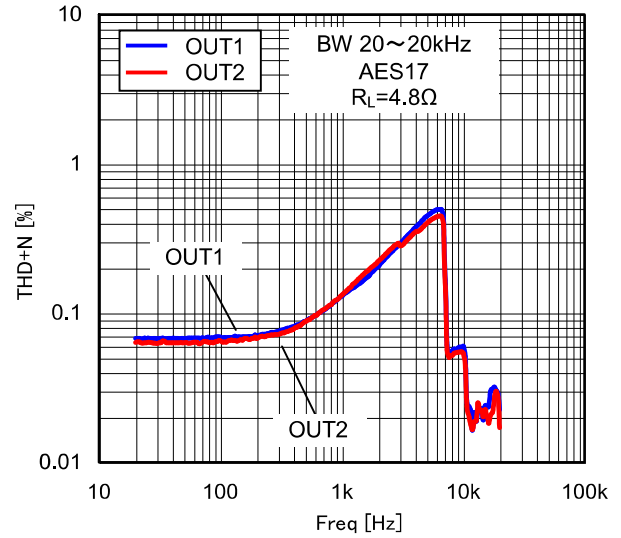
Figure 42. THD+N vs Freq (4.8 \Omega )
