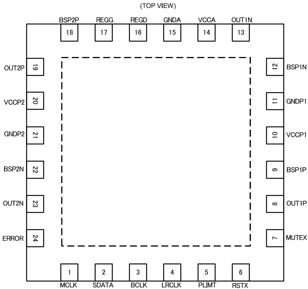
Figure 2. Pin Configuration
