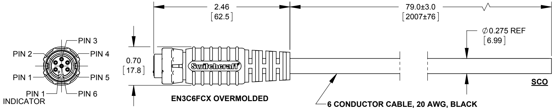
PIN CALLOUT VIEW FROM MATING SIDE OF CONNECTOR
