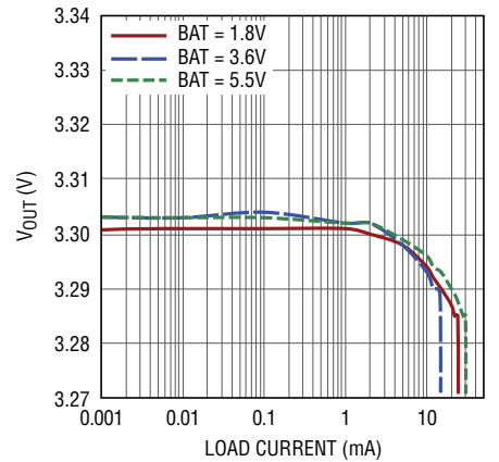
Buck-Boost Load Regulation, V_{OUT} = 3.3\text{V} , 100\text{mA } I_{PEAK} Setting
