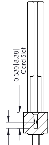
SECTION A-A 0.125 [3.18] Point of Contact
