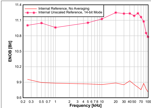
Figure 8-30. ENOB vs. Input Frequency
