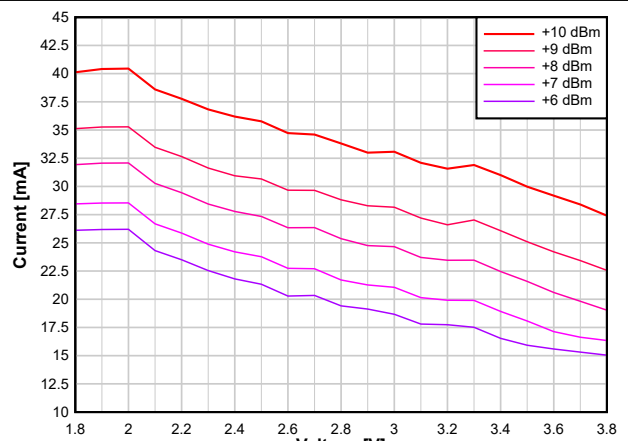
Figure 8-13. TX Current vs. Supply Voltage (VDD5) (BLE 1 Mbps, 2.44 GHz, +10 dBm PA)
