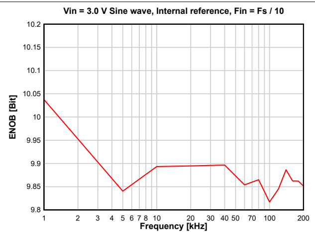
Figure 8-31. ENOB vs. Sampling Frequency
