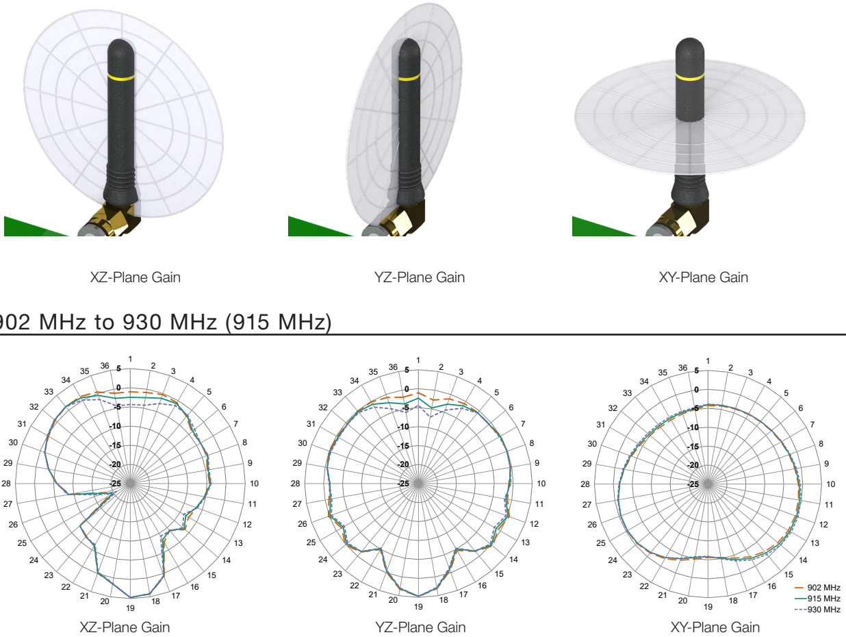
Figure 8. ANT-916-CW-RCS-ccc Radiation Patterns
