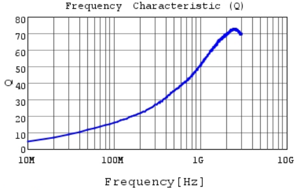
LQG15WZ3N5C02 Q
