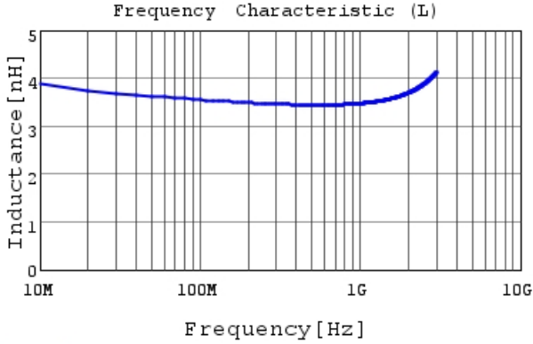
LQG15WZ3N5C02 L
