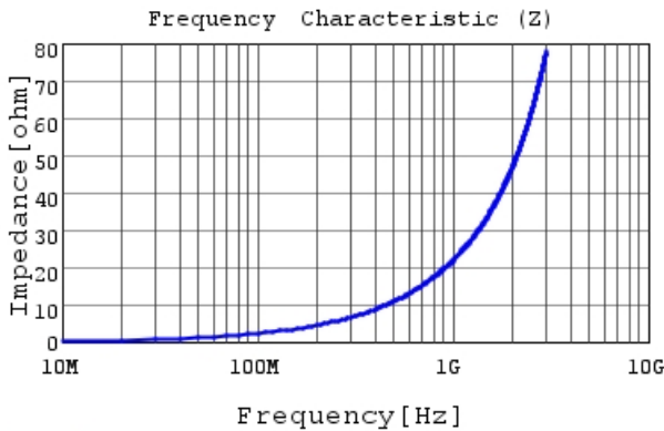
LQG15WZ3N5C02 |Z|
