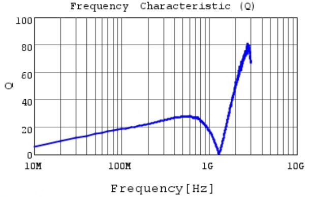
LQG15WHR10J02 Q
