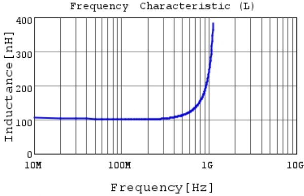
LQG15WHR10J02 L
