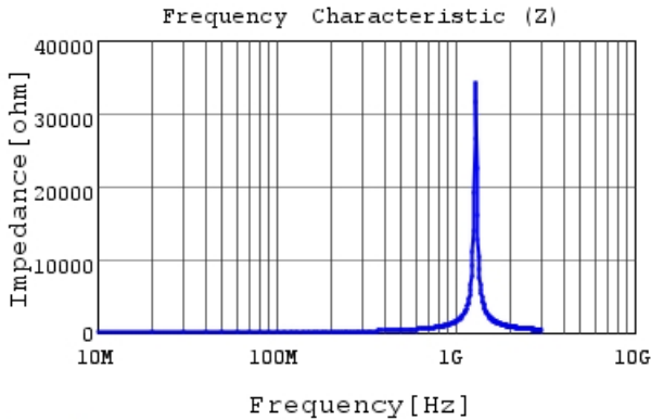
LQG15WHR10J02 |Z|
