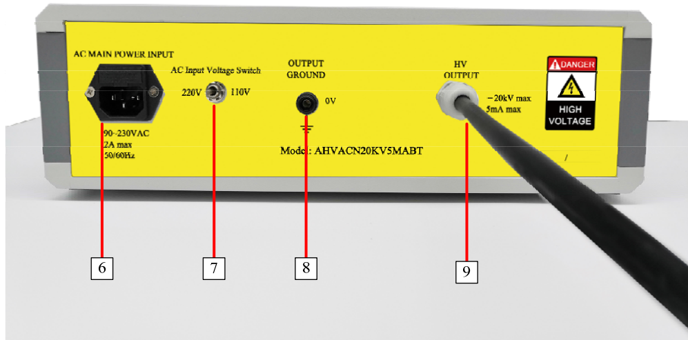
Figure 3. Front Panel
