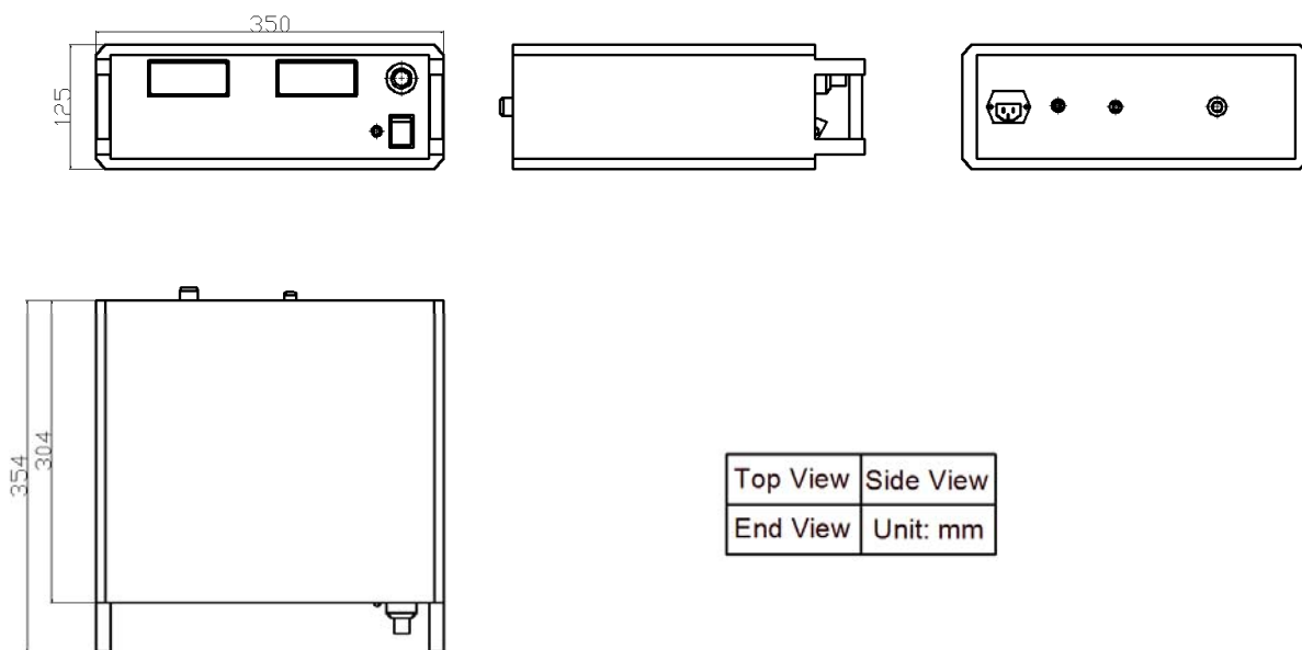
Figure 7. Dimensions for AHVACN20KV5MABT
