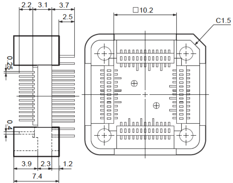
< Bottom view >
