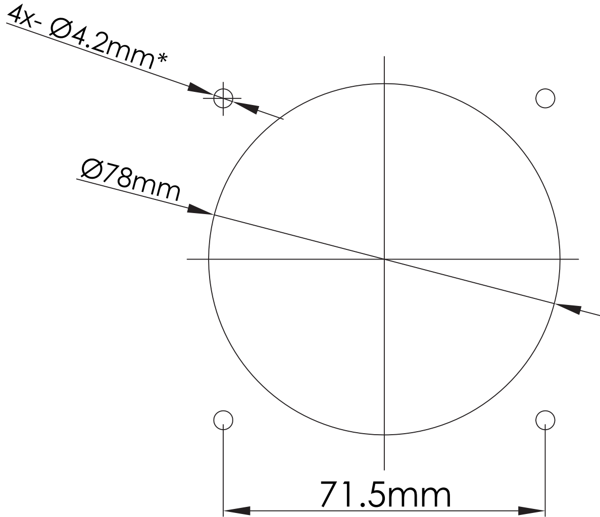
80mm Fans Panel Cutout Diagram
