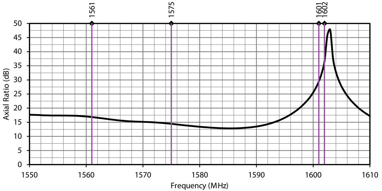
Figure 9. ANT-GNRM-L15A Series Antenna Axial Ratio, L1 Band
