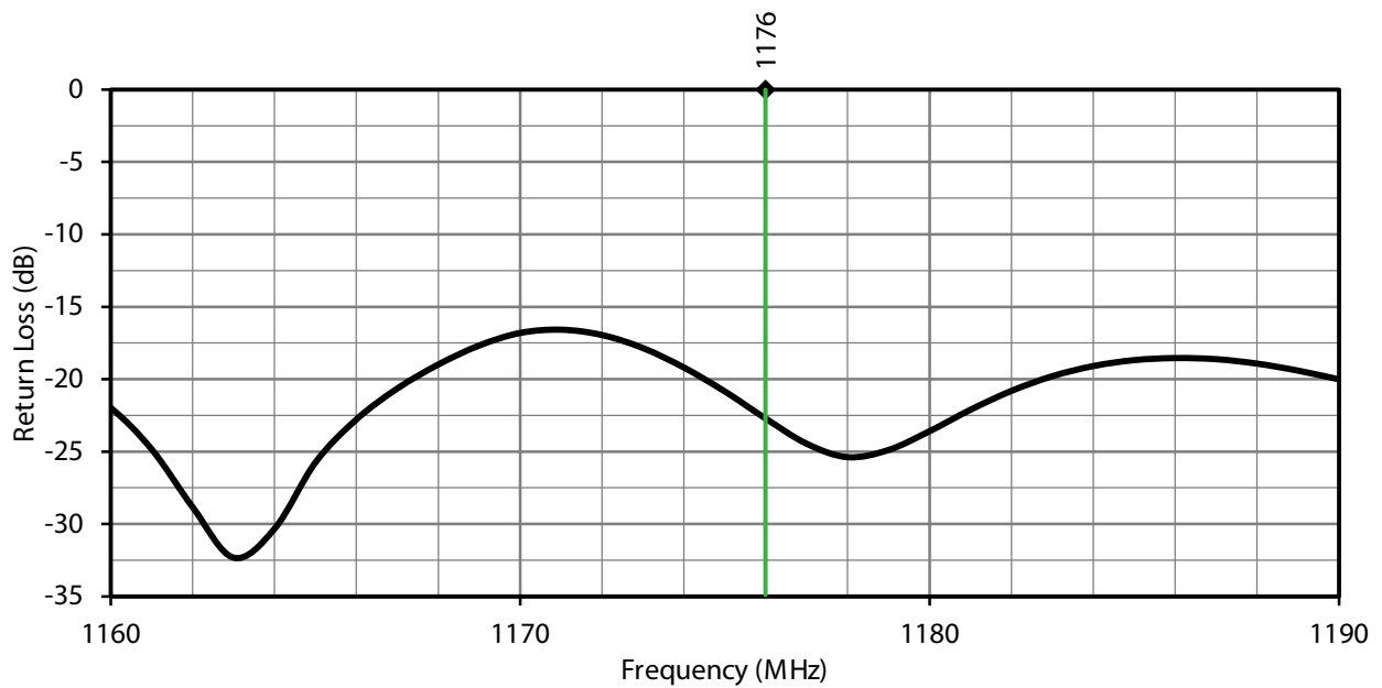
Figure 6. ANT-GNRM-L15A Series Antenna Return Loss, L5 Band
