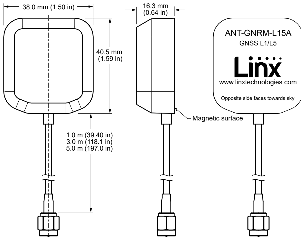
Figure 1. ANT-GNRM-L15A Series Antenna Dimensions
