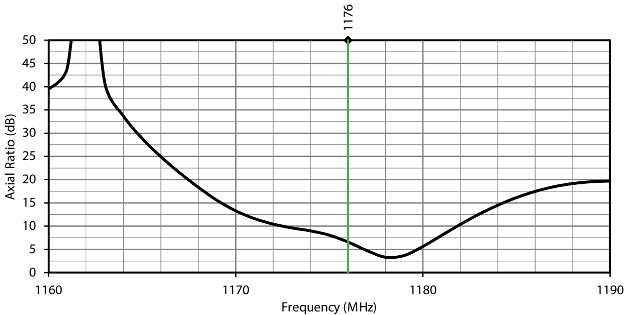
Figure 10. ANT-GNRM-L15A Series Antenna Axial Ratio, L5 Band
