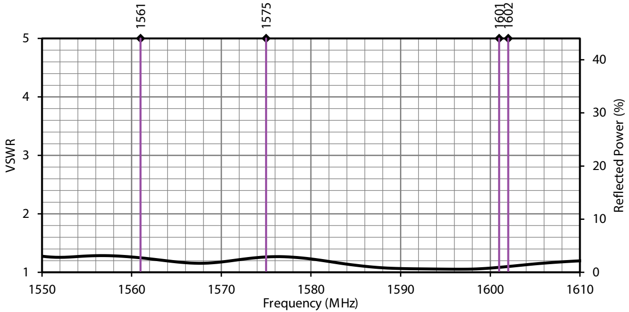
Figure 3. ANT-GNRM-L15A Series Antenna VSWR, L1 Band
