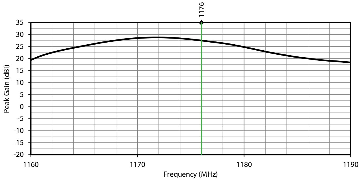
Figure 8. ANT-GNRM-L15A Series Antenna Peak Gain, L5 Band
