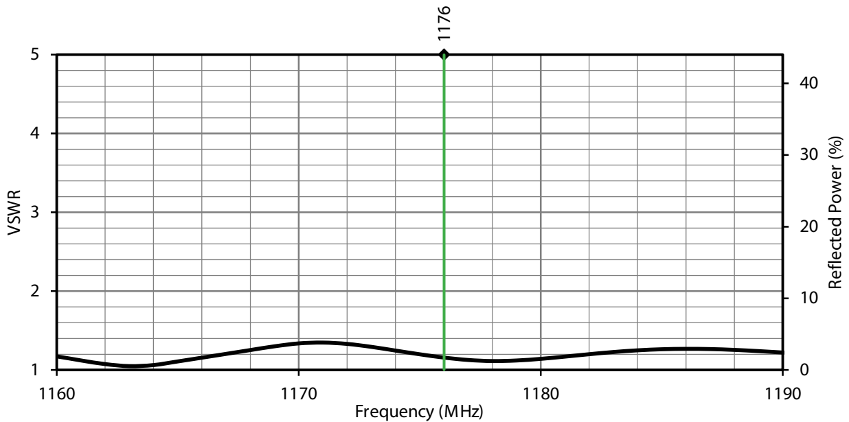
Figure 4. ANT-GNRM-L15A Series Antenna VSWR, L5 Band
