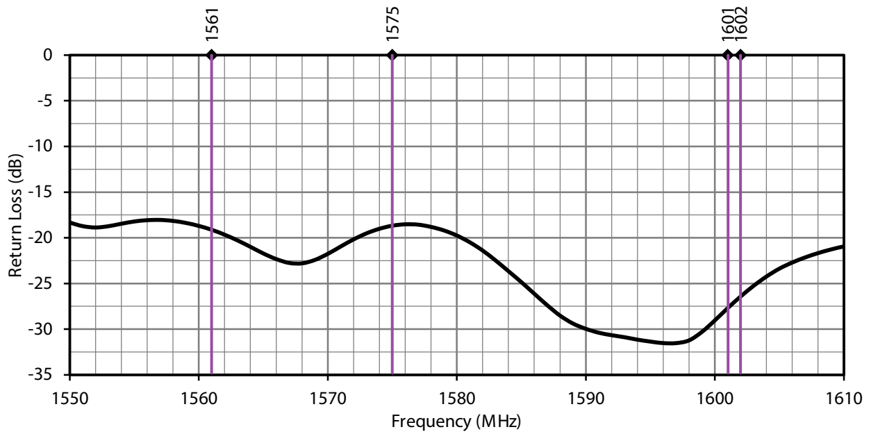
Figure 5. ANT-GNRM-L15A Series Antenna Return Loss, L1 Band
