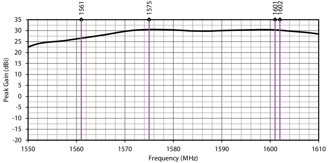
Figure 7. ANT-GNRM-L15A Series Antenna Peak Gain, L1 Band
