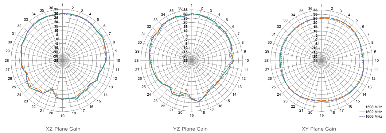
Figure 11. ANT-GNRM-L15A Series Antenna Radiation Patterns
