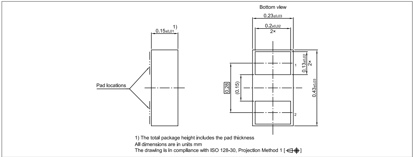
Figure 12 Package outline
