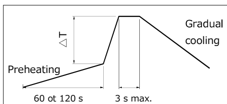
Recommended profile of Hand soldering (Ex.)
