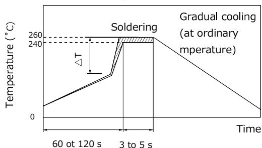
Recommended profile of Flow Soldering (Ex.)
