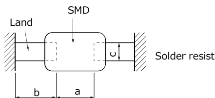
Recommended Land Dimensions(Ex.)
