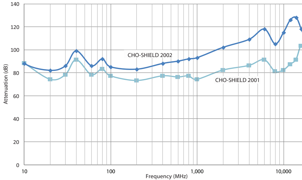
Figure 2: Shielding Effectiveness*
