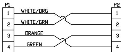
WIRING DIAGRAM
