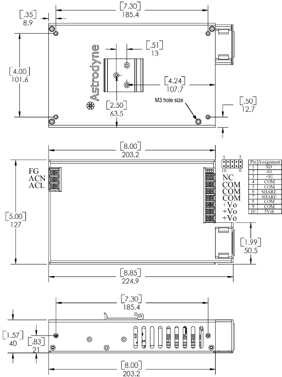
Din-rail with Fan (PMK450S-xxD) :
