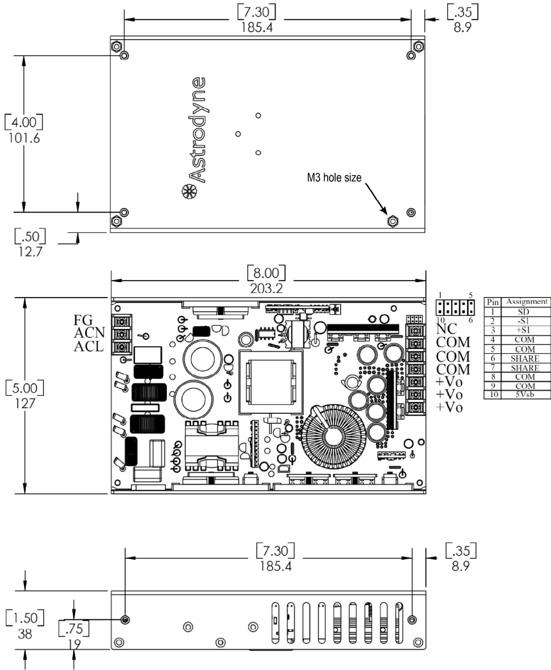
U-Bracket (PMK450S-xxU)
