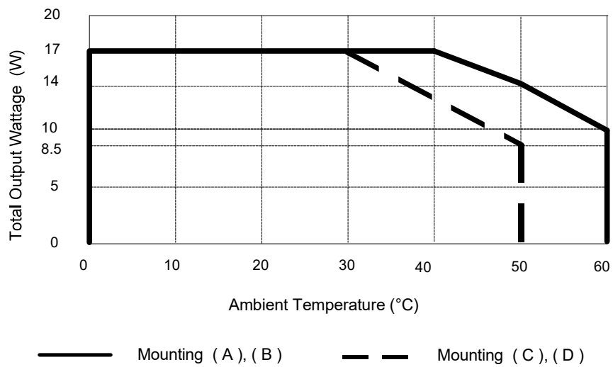
OUTPUT DERATING CURVE Convection Cooling
