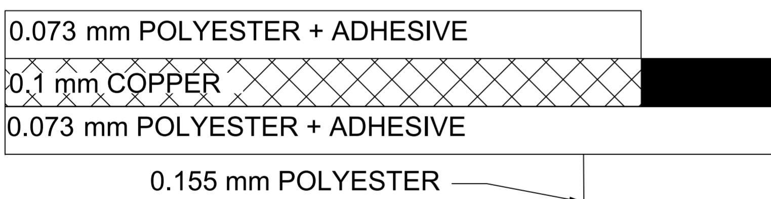
CROSS-SECTION
