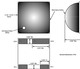
Fig. 8 4-Lead Surface Mounted Ceramic Chip Carrier
