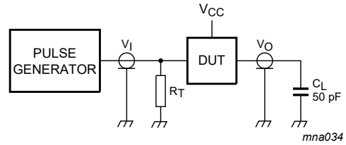
Fig. 6. Test circuit for measuring switching times Test data is given in Table 8 . Definitions for test circuit: C_L = Load capacitance including jig and probe capacitance; R_T = Termination resistance should be equal to output impedance Z_o of the pulse generator.
