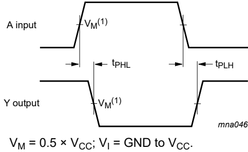
Fig. 5. The input (A) to output (Y) propagation delay times
