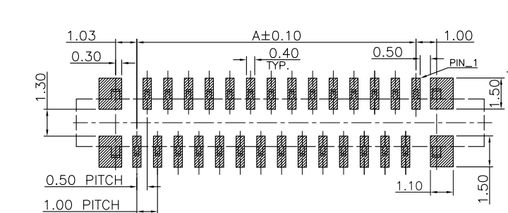
P.C.B LAYOUT A TYPE (REFERENCE) TOL:±0.05
