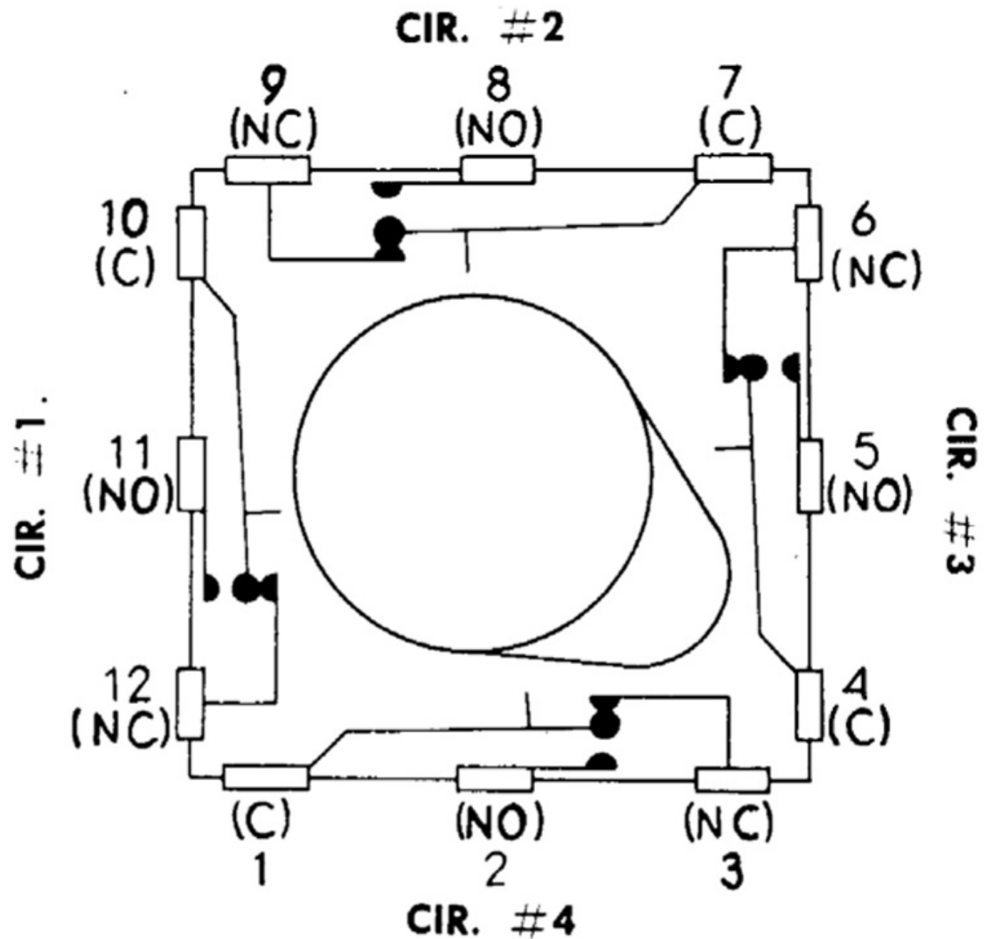
BOTTOM VIEW — SEPARATE MOTOR LEADS NOT SHOWN
