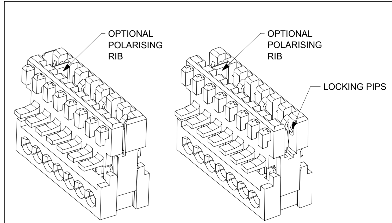
OPTION WITH SLOTTED END WALLS AND LOCKING PIPS.
