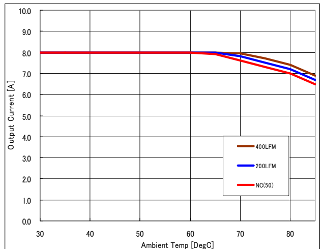
Fig.10: Output current vs. ambient temperature and air velocity at 12Vin, 0.8Vout
