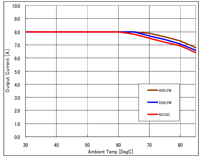
Fig.8: Output current vs. ambient temperature and air velocity at 12Vin, 1.2Vout
