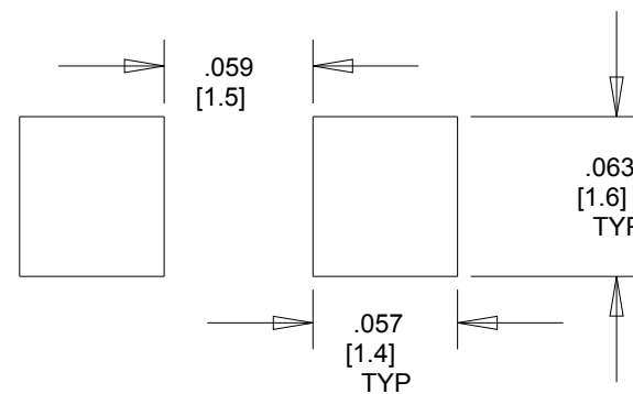
SOLDER PAD LAYOUT
