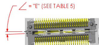
INITIAL Z AXIS ANGULAR MISALIGNMENT
