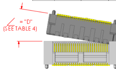
INITIAL Y AXIS ANGULAR MISALIGNMENT
