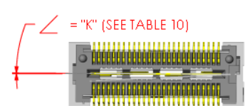
FINAL Z AXIS ANGULAR MISALIGNMENT
