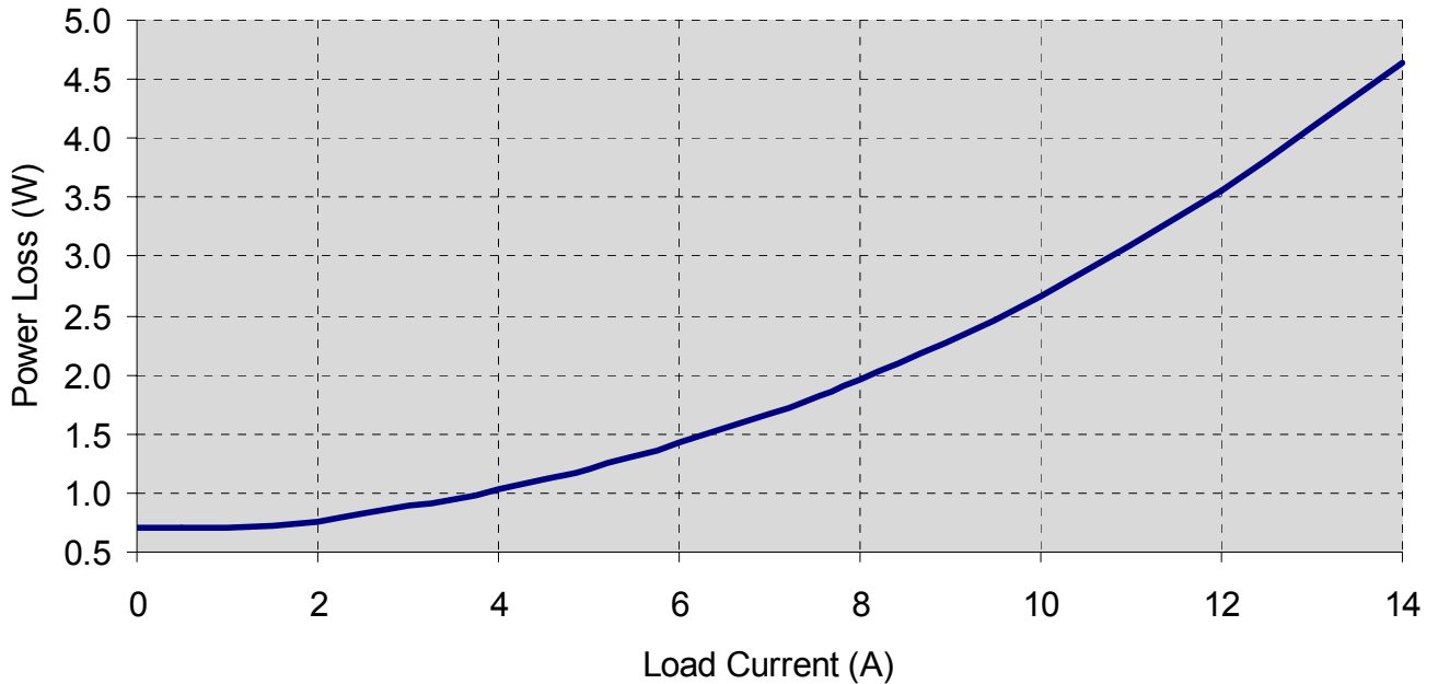
Fig. 16: Power Loss versus load current
