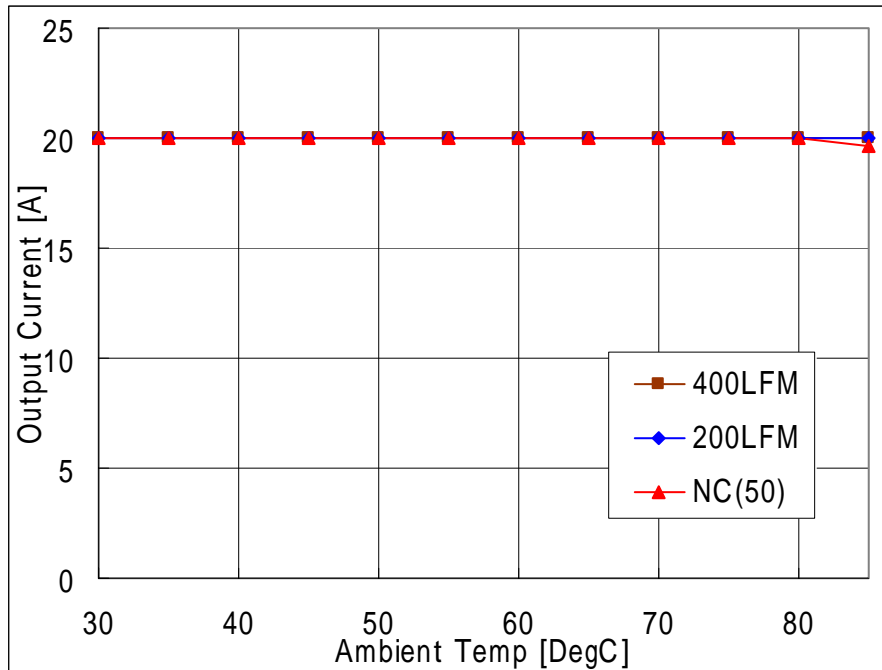
Fig-3.3V-1: Available load current vs. ambient temperature and airflow rates for V_{out}=3.3V with V_{in}=12.0V . Maximum component temperature 120^{\circ}C
