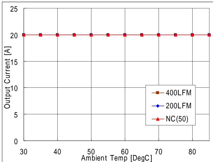
Fig-1.5V-1: Available load current vs. ambient temperature and airflow rates for V_{out}=1.5V with V_{in}=12.0V . Maximum component temperature 120^{\circ}C
