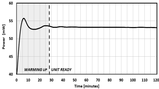
FIG. 7: WARM-UP TIME
