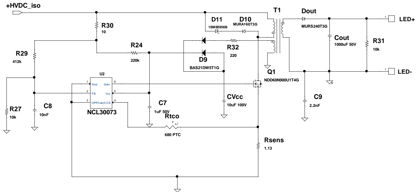
Figure 2. Main Schematic
