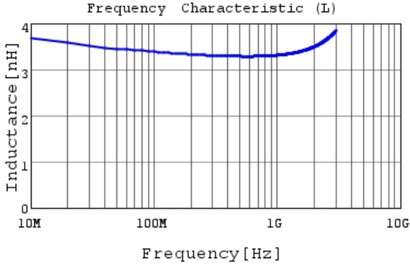
LQG15WZ3N4S02 L
