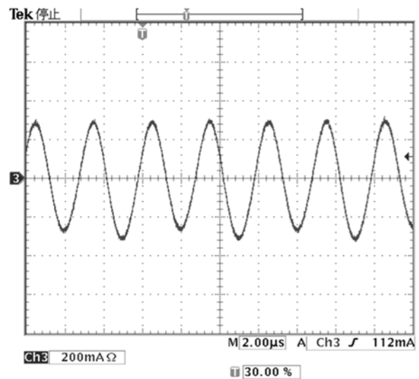
Fig.10: Input reflected ripple current, I_c (200mA/div), measured through 1uH at the source at full rated load current and V_{in}=48V . Time scale: 2us/div.
