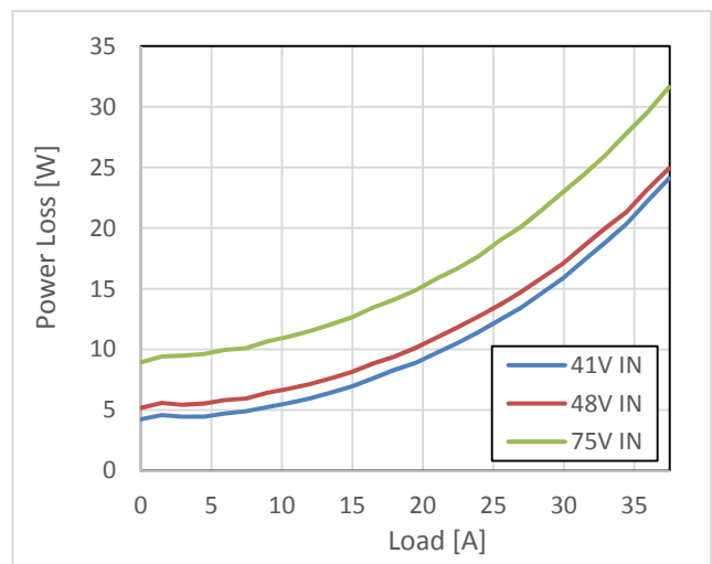
Fig.3: Power Loss vs. load current and input voltage for power module mounted horizontally with airflow 400LFM (2.0m/s) and Ta=25°C.
