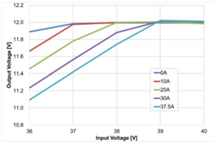
Fig.13: Vout vs. Vin at output voltage setting = 12 V. Power supply module 600 LFM (3.0 m / s) and Ta = 25 ° C horizontally mounted
