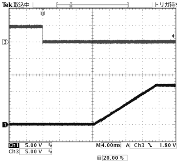
Fig.4: Turn-on transient at full rated load current (resistive) 198uF cap at Vin=48V, triggered via ON/OFF pin. Top trace: ON/OFF signal (5V/div). Bottom trace: output voltage (5V/div). Time scale: 4ms/div
