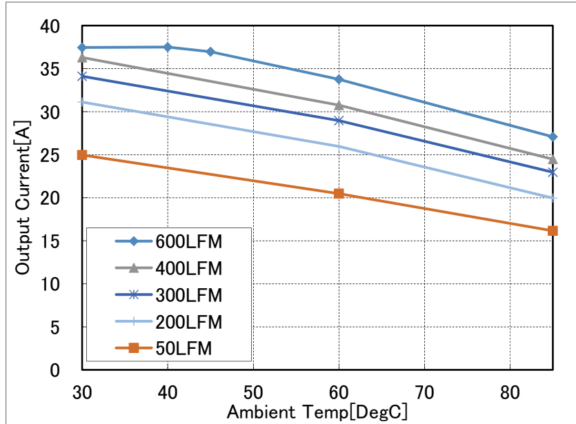
Fig.1-a: Available load current vs. ambient temperature and airflow rates for Vin=48V with baseplate. Airflow is from Pin 3 to Pin 1. Maximum component temperature \leq 125^{\circ}\text{C}
