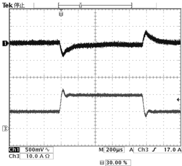
Fig.6: Output voltage response to load current step-change (25%⇒50%) at Vin=48V. Top trace: Output voltage (500mV/div). Bottom trace: load current (10A/div). Current slew rate: 0.5A/μs. Co=132uF ceramic and 1500uF Electrolytic, Time scale: 200us/div
