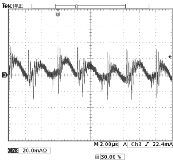
Fig.9: Input reflected ripple current, I_s (20mA/div), measured through 1uH at the source at full rated load current and V_{in}=48V . Time scale: 2us/div.
