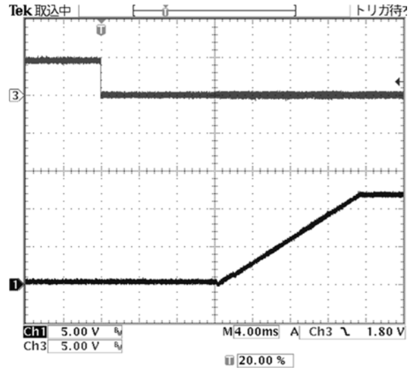
Fig.5: Turn-on transient at full rated load current (resistive) plus 2200uF at Vin=48V, triggered via ON/OFF pin. Top trace: ON/OFF signal (5V/div). Bottom trace: output voltage (5V/div). Time scale: 4ms/div
