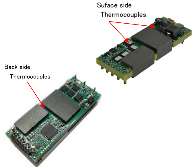
Fig. G: Location of thermocouples for thermal testing
