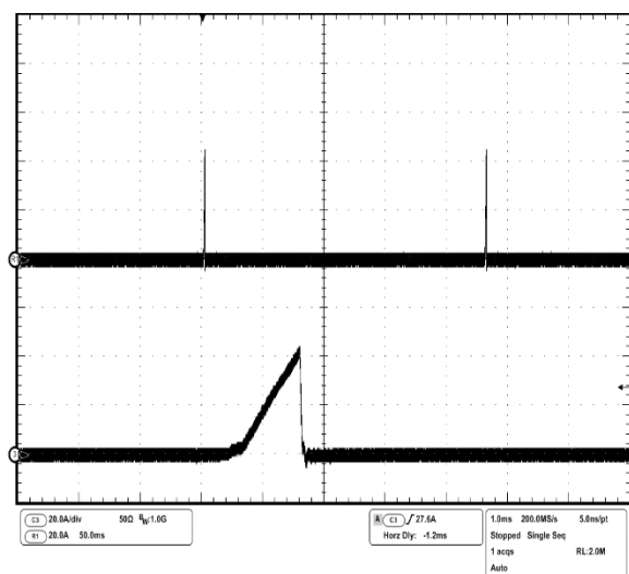
Fig.12: Load current (top trace, 20A/div, 50ms/div) into a 10mΩ short circuit during restart, at V_{in} = 48V . Bottom trace (20A/div, 1ms/div) is an expansion of the top trace.
