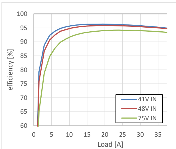
Fig.2: Efficiency vs. load current and input voltage for power module mounted horizontally with airflow 400LFM (2.0m/s) and Ta=25°C.
