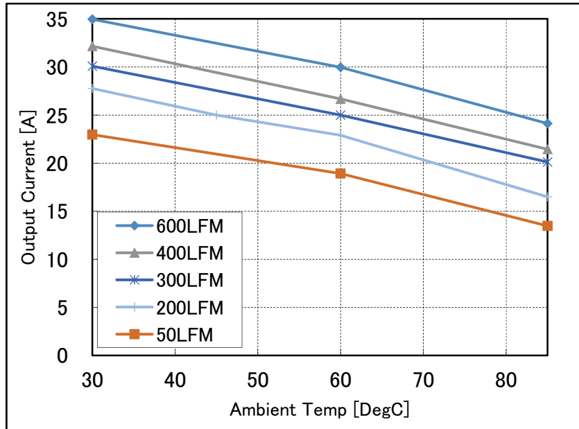
Fig.1-b: Available load current vs. ambient temperature and airflow rates for Vin=48V without baseplate (open frame). Airflow is from Pin 3 to Pin 1. Maximum component temperature \leq 125^{\circ}\text{C}
