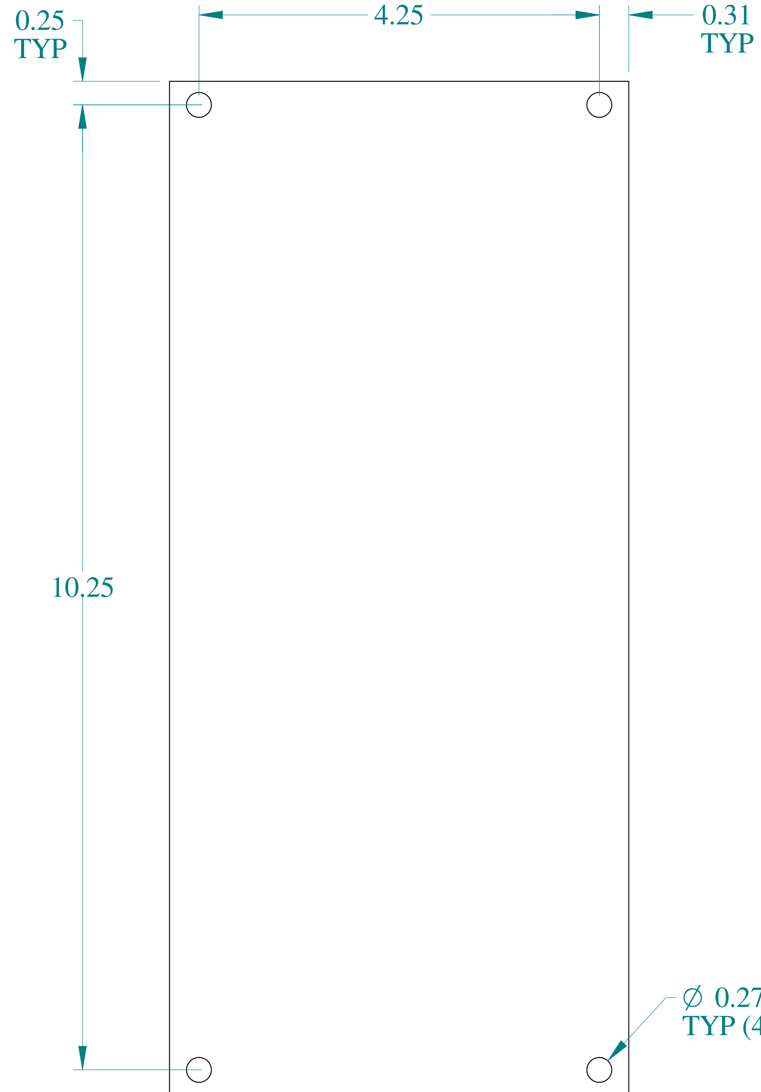
FRONT VIEW
