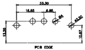
3W3 / 3WK3
