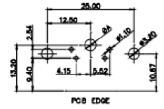
7W2 Male/Female
