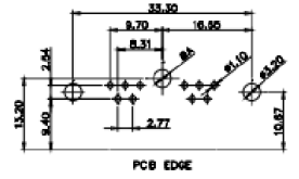
17W2 Male/Female
