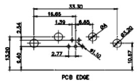
11W1 Male/Female
