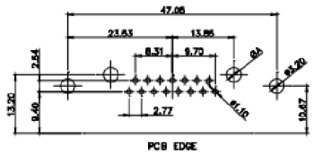
17W2 Male/Female
