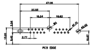
21W1 Male/Female
